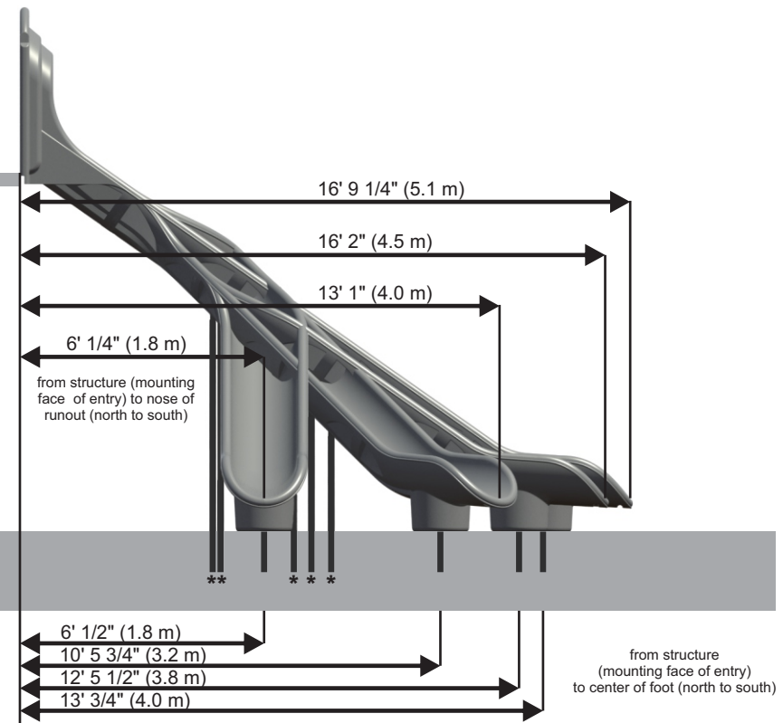
Side Views
