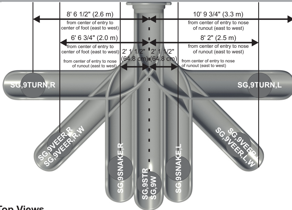
Top Views
