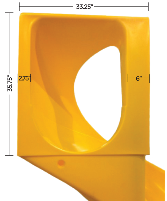
Slide entrance dimensions for installation purpose
