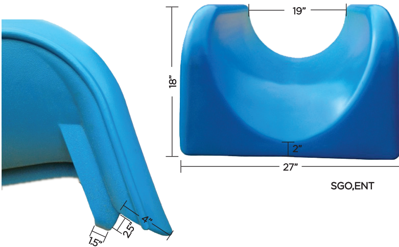
SGO,ENT SIDE VIEW
